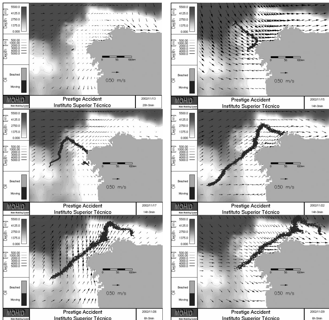
Figure 8 MeteoMohid simulation of the track of the first spill taking into account the slope current at different times (in the figures). Notice the tail does not touch the southern Galician coast.
